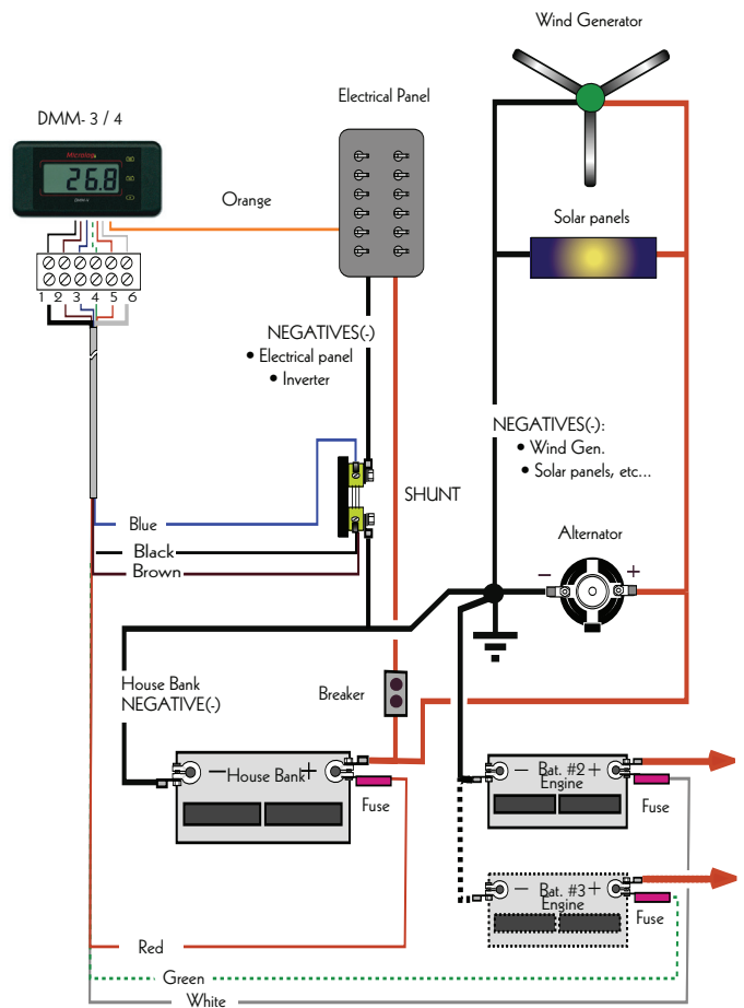
Figure 3: Shunt Installation to monitor the discharge current
