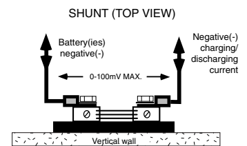
Shunt installation
