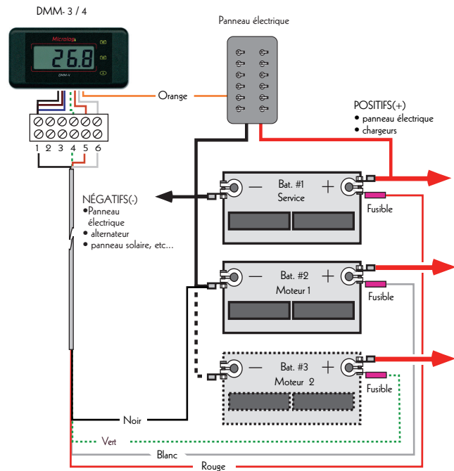
Figure 1: Installation sans shunt
